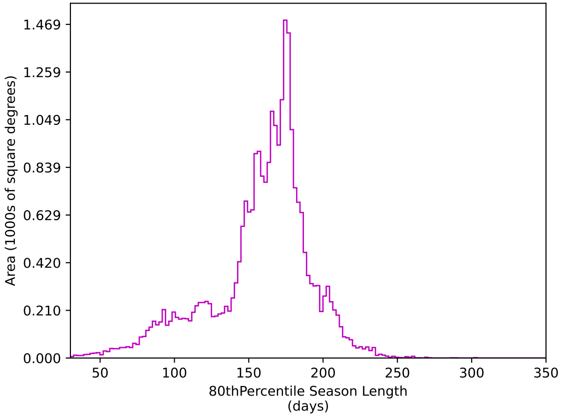
too_elab_r64_d3_griz_v3.4_10yrs All sky z band: 80thPercentile Season Length
