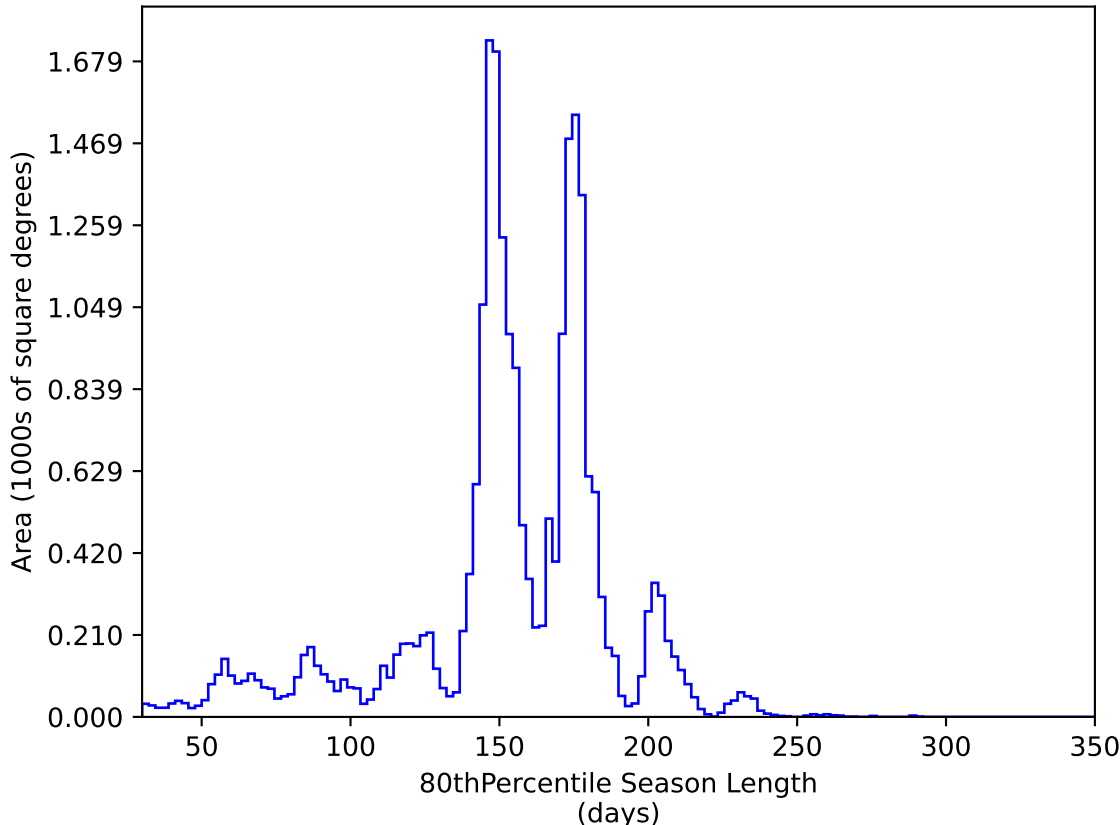
too_elab_r64_d3_griz_v3.4_10yrs All sky y band: 80thPercentile Season Length
