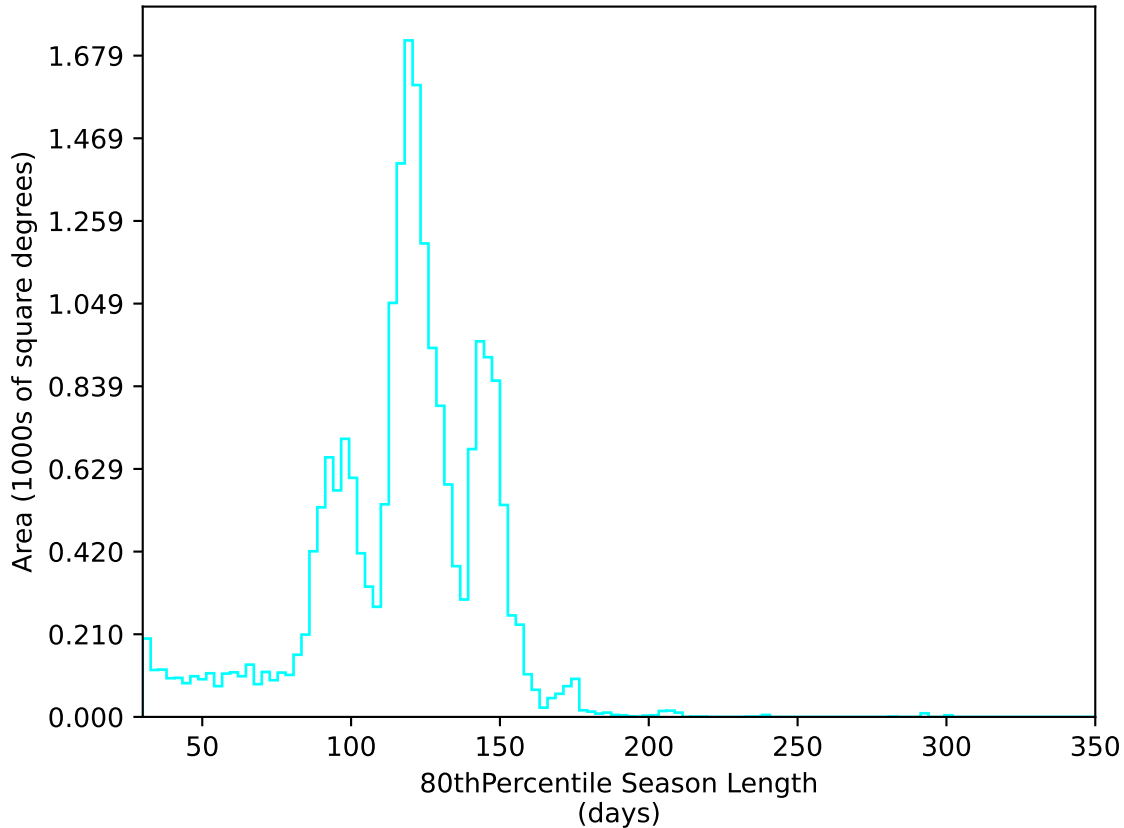
too_elab_r64_d3_griz_v3.4_10yrs All sky u band: 80thPercentile Season Length
