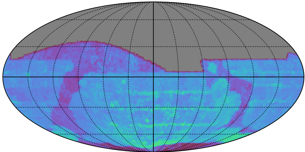
too_elab_r64_d3_griz_v3.4_10yrs All sky r band: 80thPercentile Season Length
