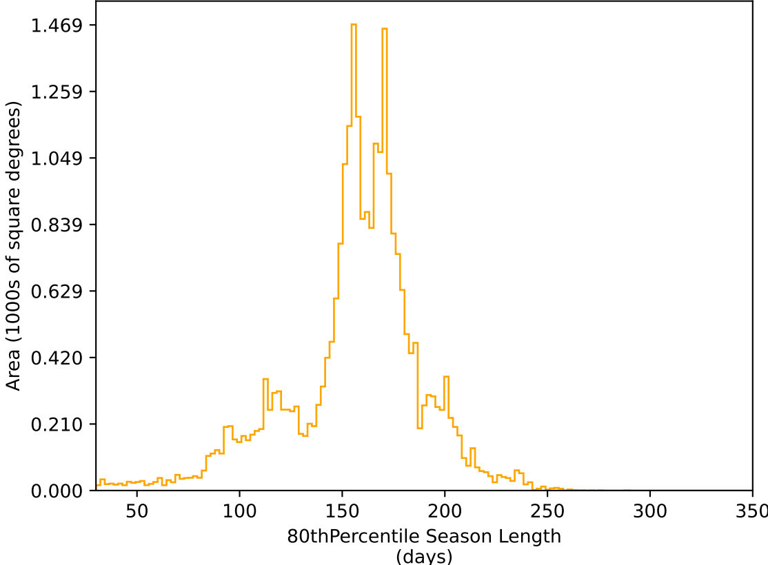
too_elab_r64_d3_griz_v3.4_10yrs All sky r band: 80thPercentile Season Length
