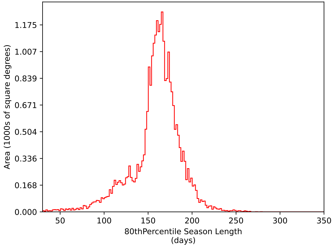
too_elab_r64_d3_griz_v3.4_10yrs All sky i band: 80thPercentile Season Length
