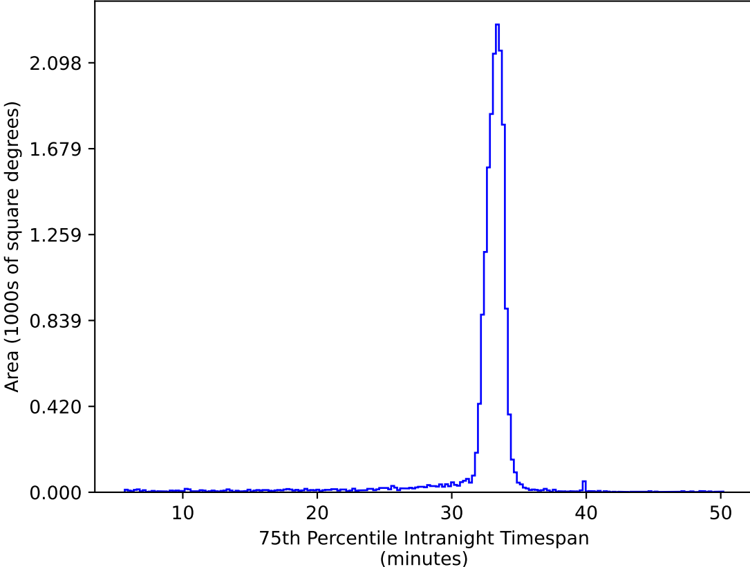
too_elab_r64_d3_griz_v3.4_10yrs WFD ug bands: 75th Percentile Intranight Timespan
