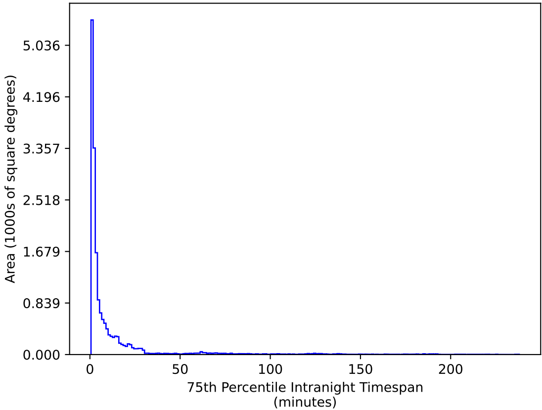
too_elab_r64_d3_griz_v3.4_10yrs WFD u band: 75th Percentile Intranight Timespan
