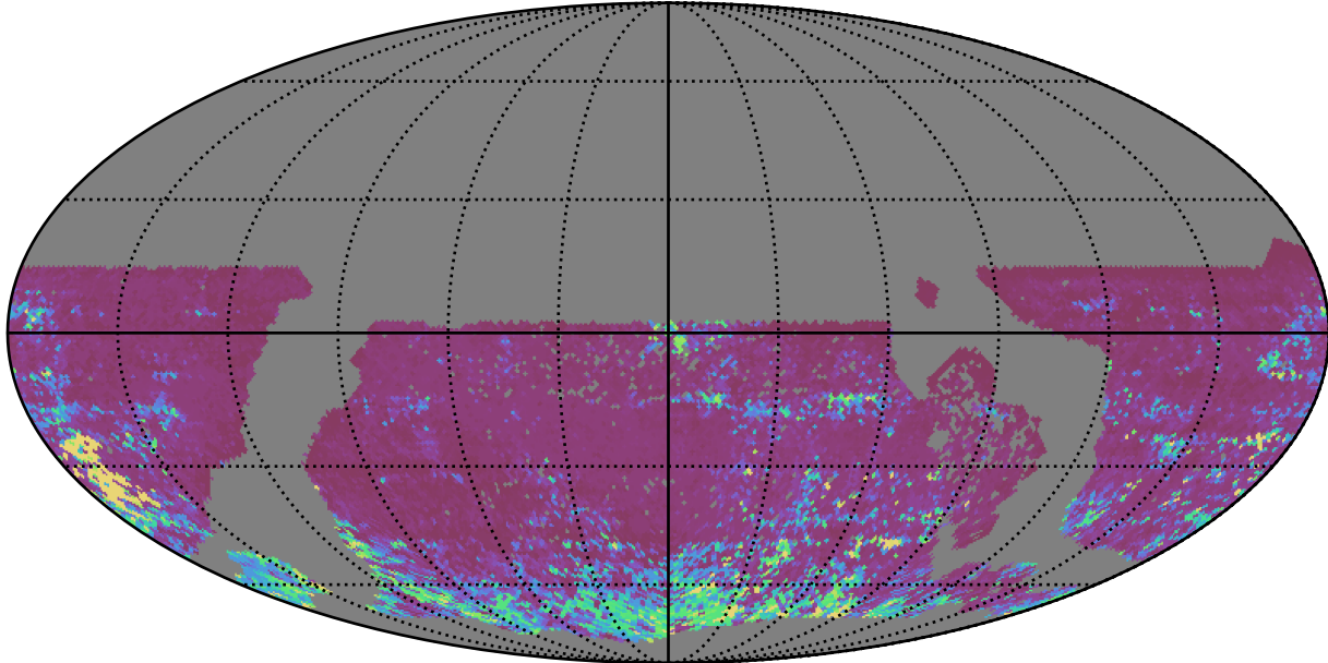
too_elab_r64_d3_griz_v3.4_10yrs WFD i band: 75th Percentile Intranight Timespan
