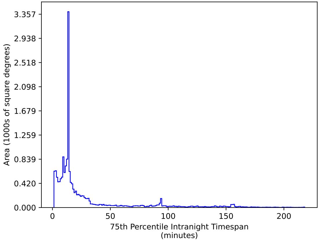
too_elab_r64_d3_griz_v3.4_10yrs WFD i band: 75th Percentile Intranight Timespan
