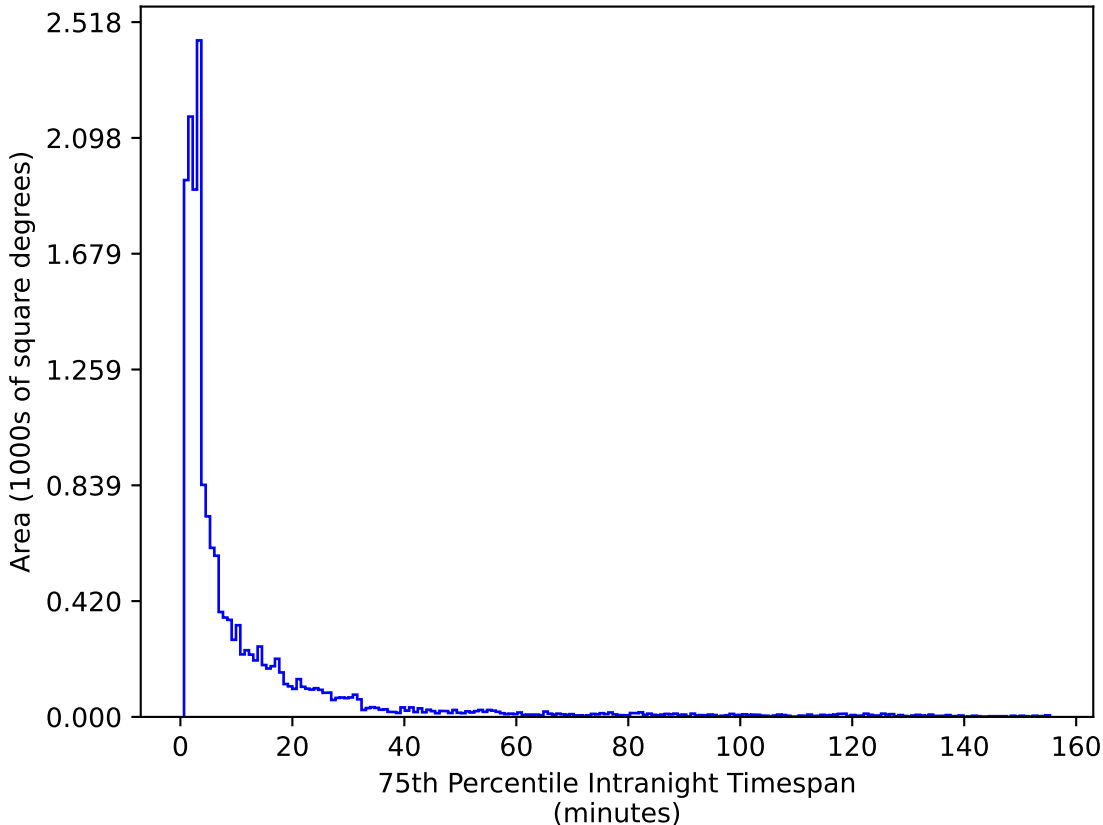
too_elab_r64_d3_griz_v3.4_10yrs WFD g band: 75th Percentile Intranight Timespan
