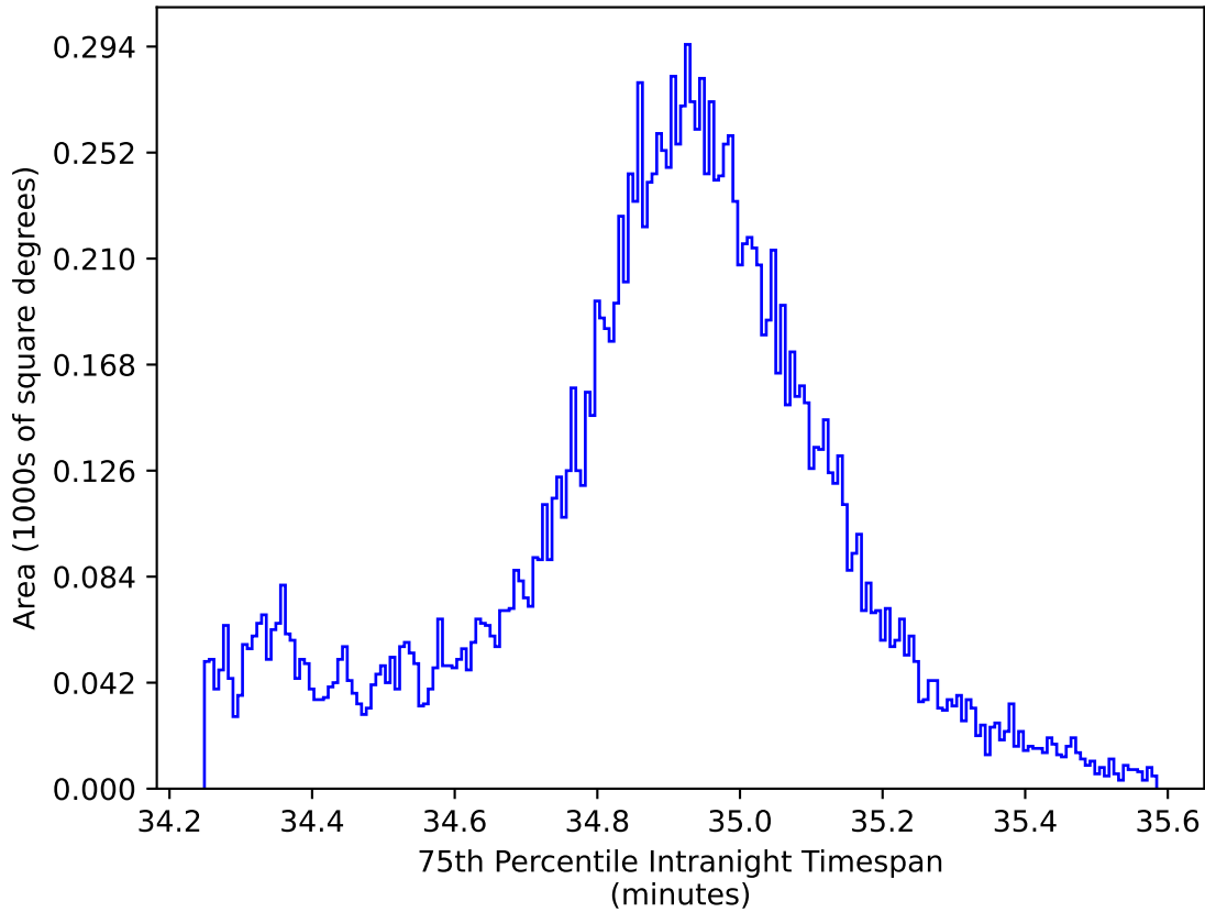
too_elab_r64_d3_griz_v3.4_10yrs WFD all bands: 75th Percentile Intranight Timespan
