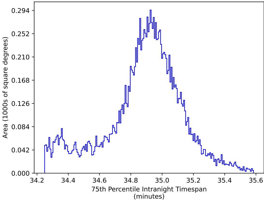
too_elab_r64_d3_griz_v3.4_10yrs WFD: 75th Percentile Intranight Timespan
