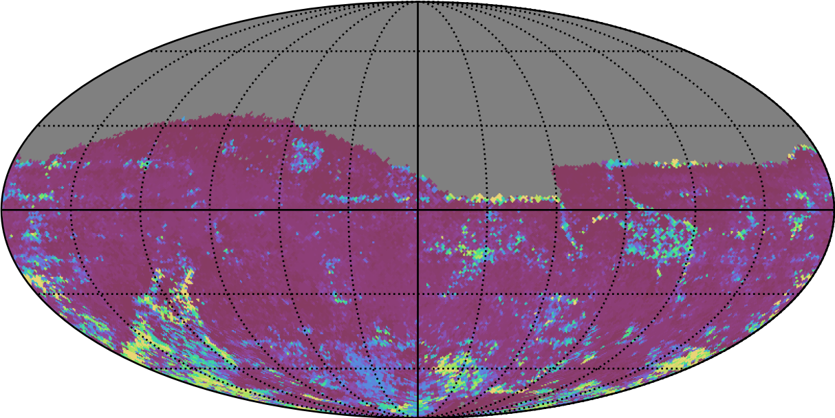
too_elab_r64_d3_griz_v3.4_10yrs All sky z band: 75th Percentile Intranight Timespan
