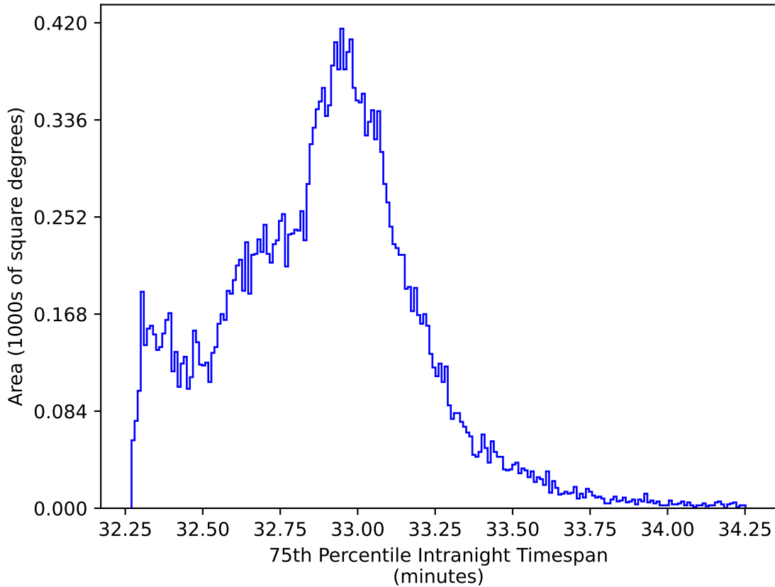
too_elab_r64_d3_griz_v3.4_10yrs All sky y band: 75th Percentile Intranight Timespan
