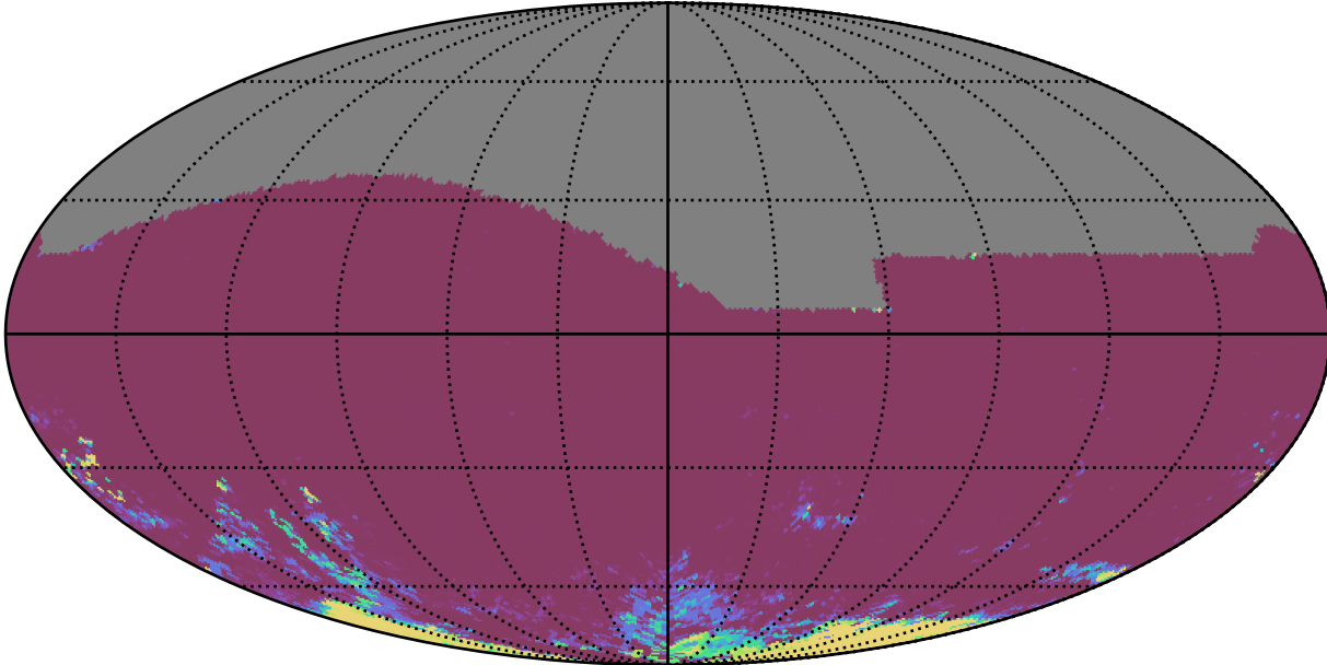
too_elab_r64_d3_griz_v3.4_10yrs All sky ri bands: 75th Percentile Intranight Timespan
