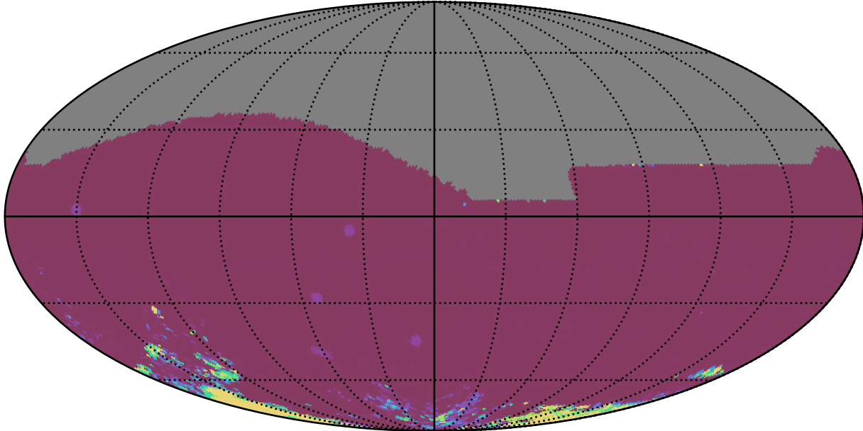
too_elab_r64_d3_griz_v3.4_10yrs All sky iz bands: 75th Percentile Intranight Timespan
