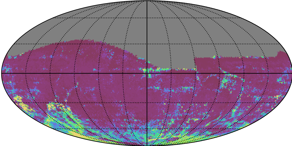
too_elab_r64_d3_griz_v3.4_10yrs All sky i band: 75th Percentile Intranight Timespan
