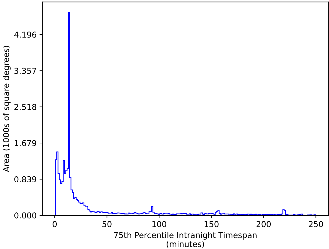
too_elab_r64_d3_griz_v3.4_10yrs All sky i band: 75th Percentile Intranight Timespan
