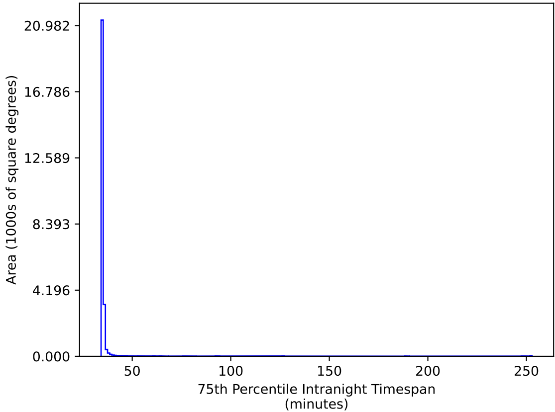
too_elab_r64_d3_griz_v3.4_10yrs All sky gr bands: 75th Percentile Intranight Timespan
