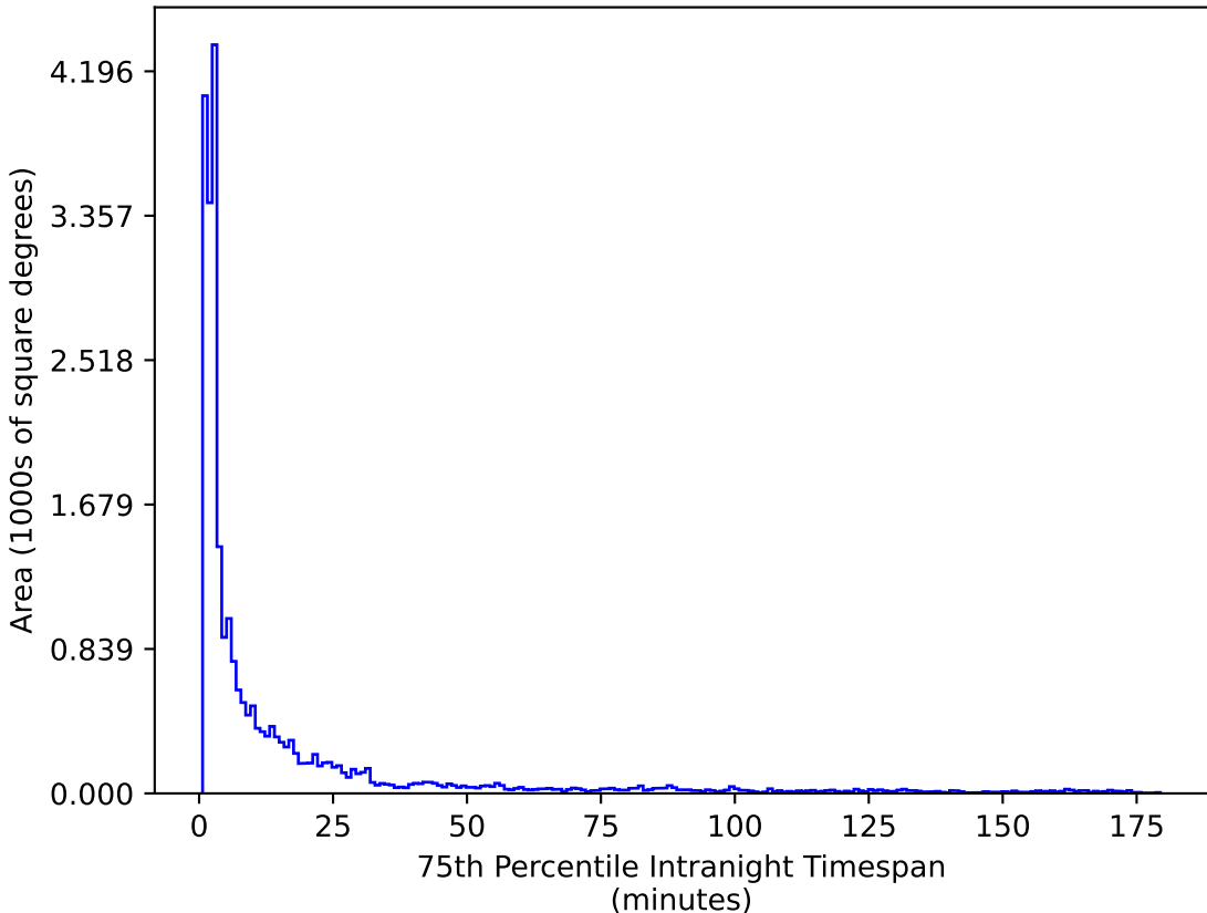
too_elab_r64_d3_griz_v3.4_10yrs All sky g band: 75th Percentile Intranight Timespan
