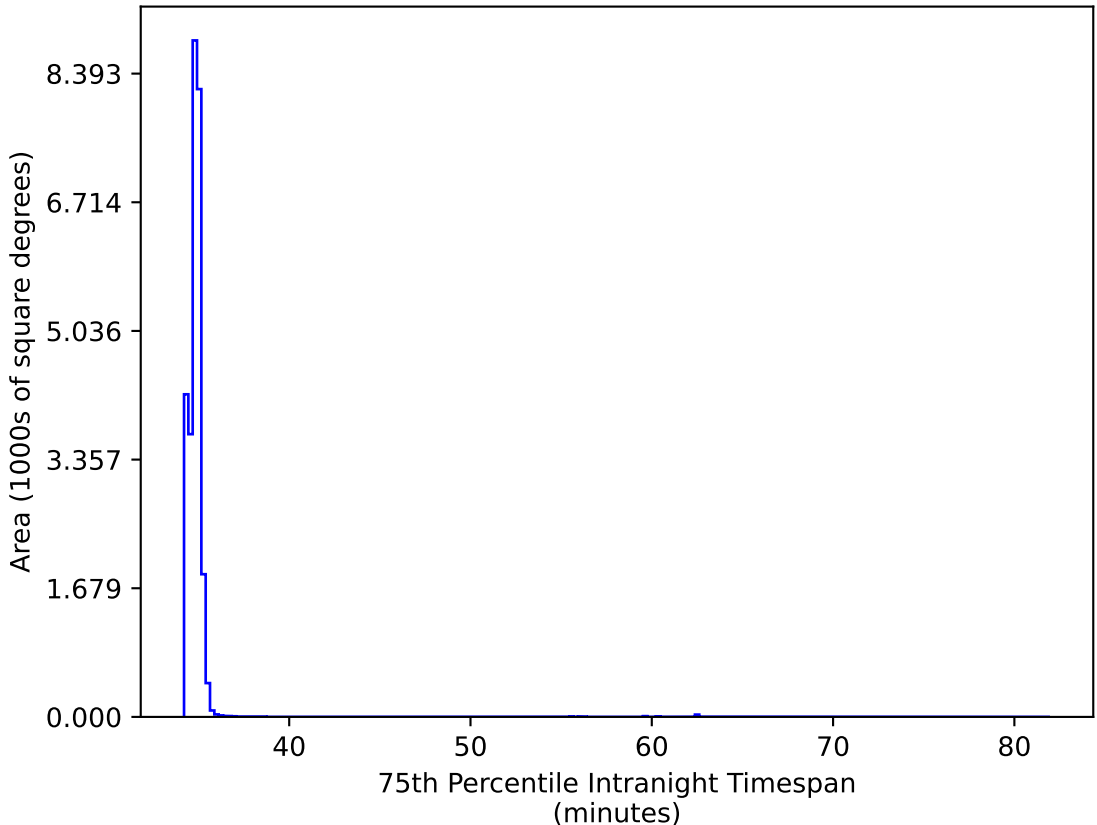
too_elab_r64_d3_griz_v3.4_10yrs All sky all bands: 75th Percentile Intranight Timespan
