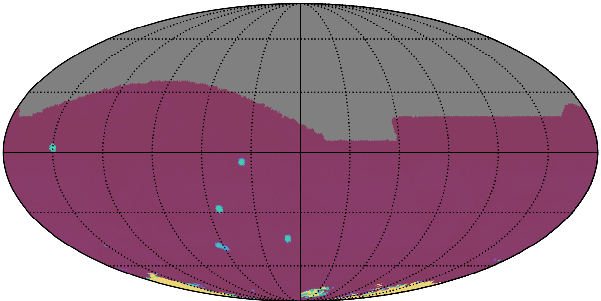
too_elab_r64_d3_griz_v3.4_10yrs All sky: 75th Percentile Intranight Timespan
