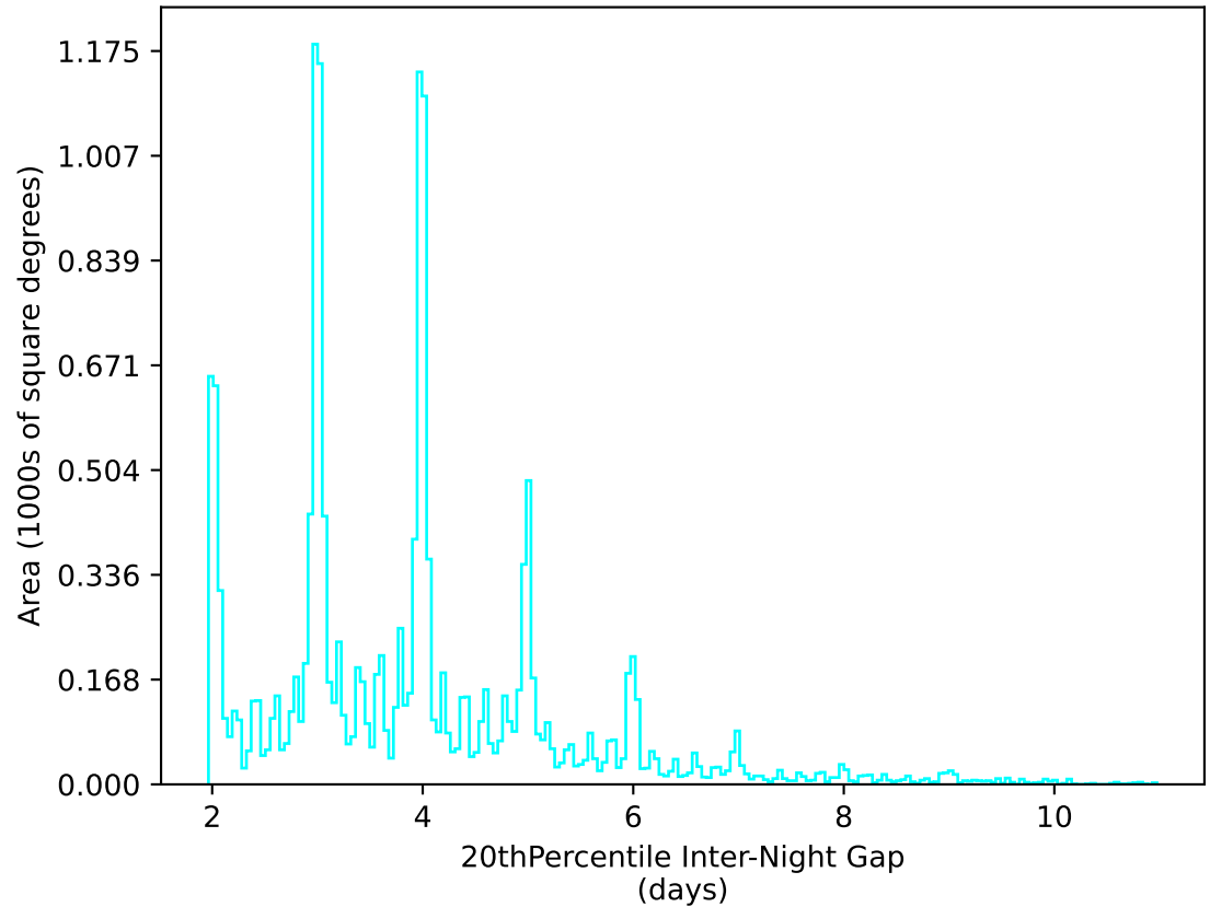
too_elab_r64_d3_griz_v3.4_10yrs WFD u band: 20thPercentile Inter-Night Gap
