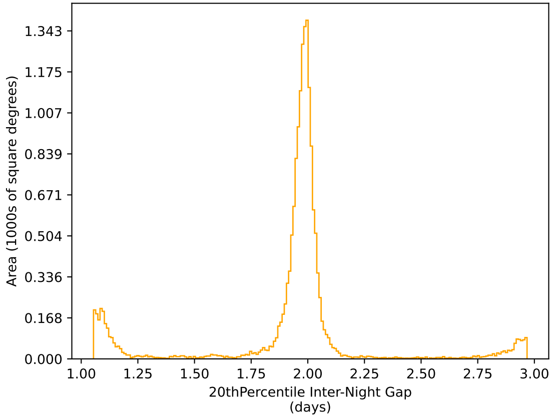
too_elab_r64_d3_griz_v3.4_10yrs WFD r band: 20thPercentile Inter-Night Gap
