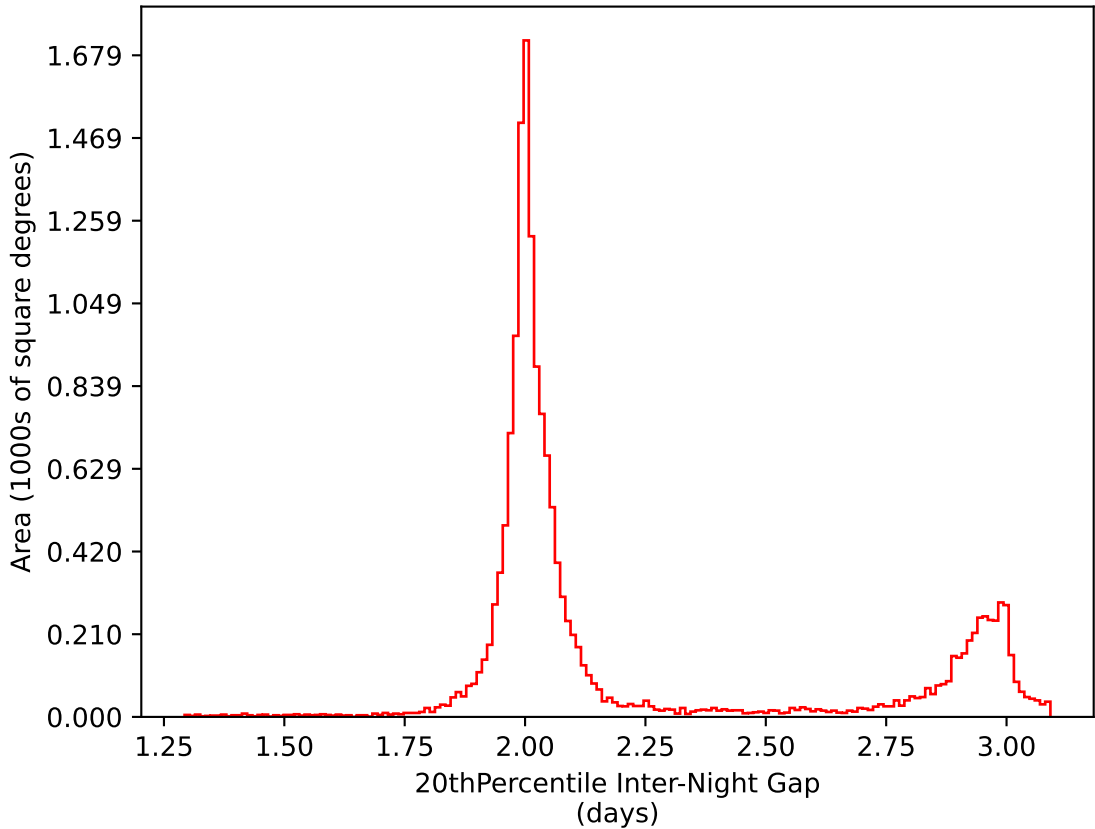
too_elab_r64_d3_griz_v3.4_10yrs WFD i band: 20thPercentile Inter-Night Gap
