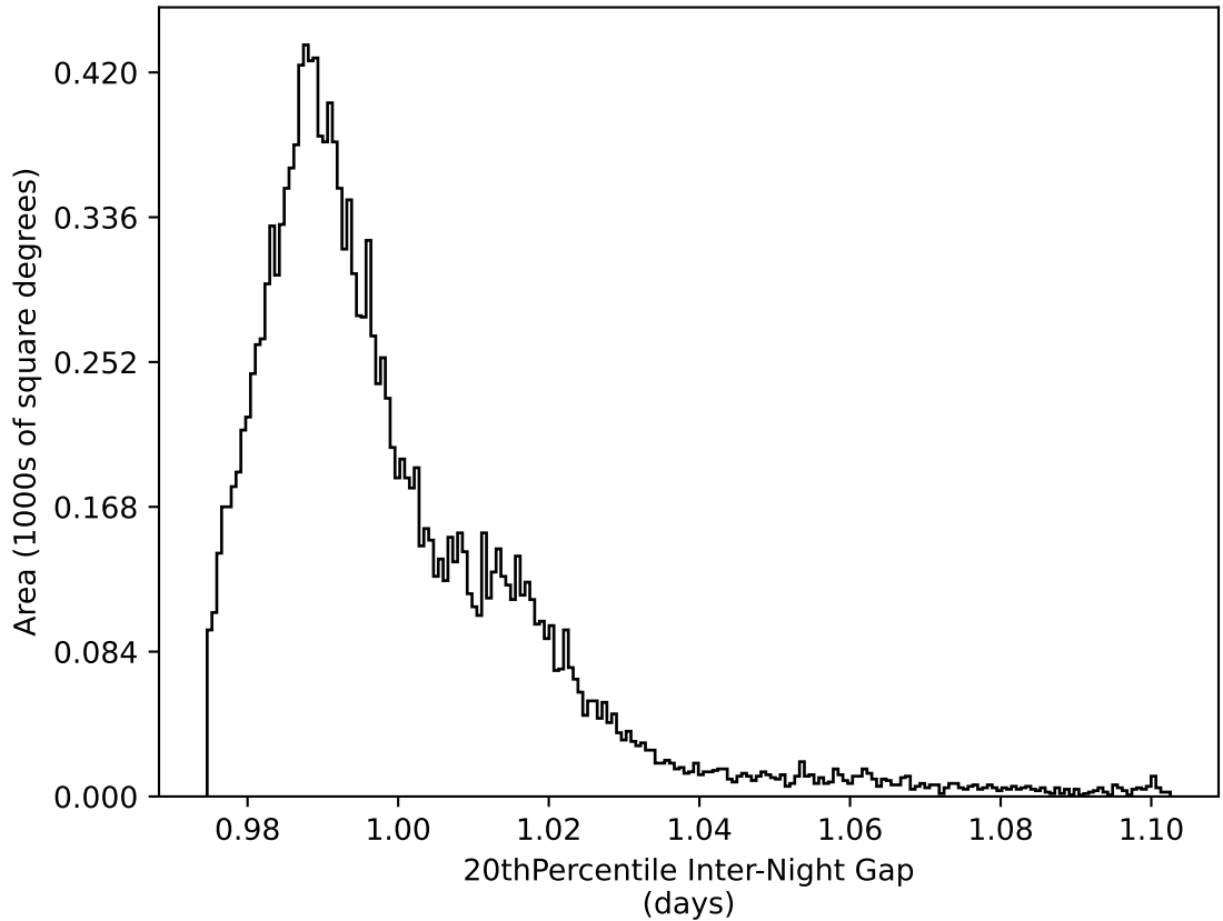
too_elab_r64_d3_griz_v3.4_10yrs WFD all bands: 20thPercentile Inter-Night Gap
