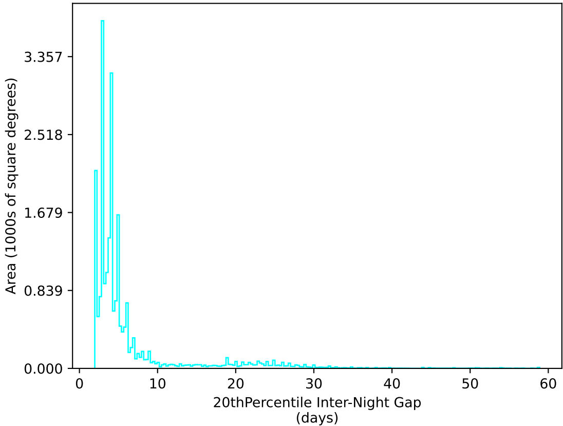
too_elab_r64_d3_griz_v3.4_10yrs All sky u band: 20thPercentile Inter-Night Gap
