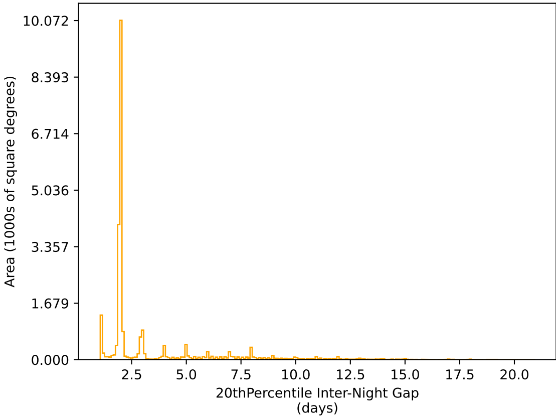
too_elab_r64_d3_griz_v3.4_10yrs All sky r band: 20thPercentile Inter-Night Gap
