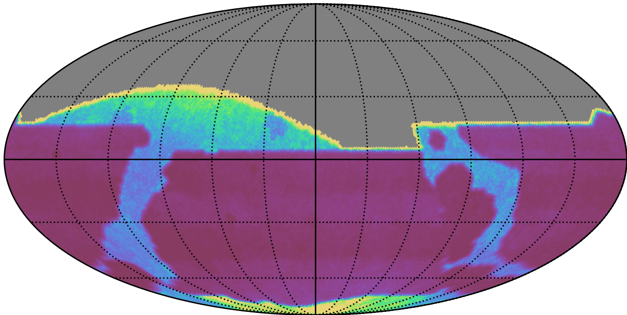
too_elab_r64_d3_griz_v3.4_10yrs : properMotion
