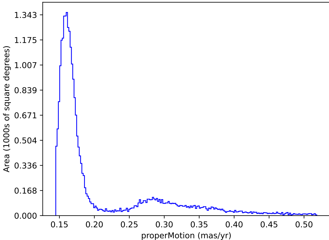
too_elab_r64_d3_griz_v3.4_10yrs : properMotion
