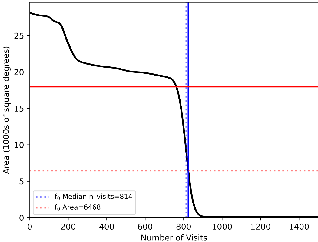
too_elab_r64_d3_griz_v3.4_10yrs : f0
