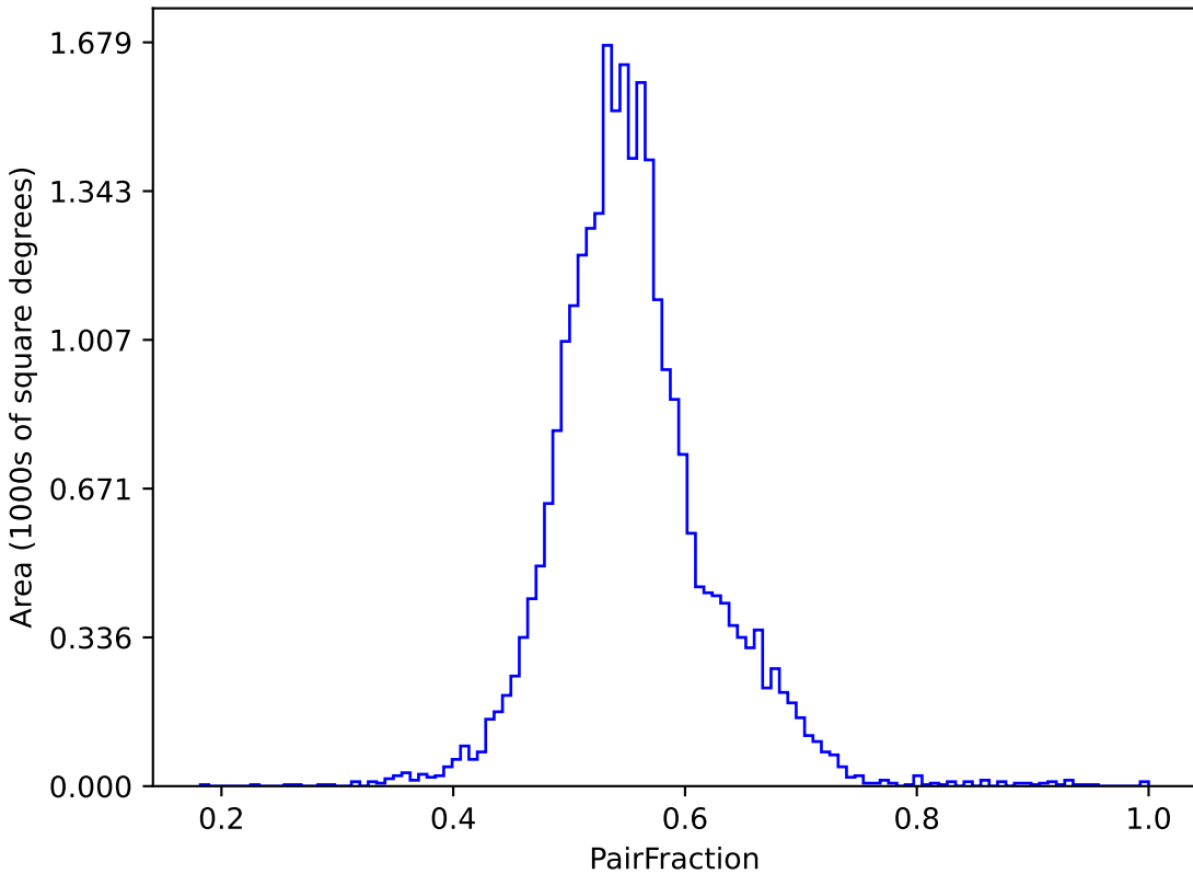
too_elab_r64_d3_griz_v3.4_10yrs (g or r or i): PairFraction
