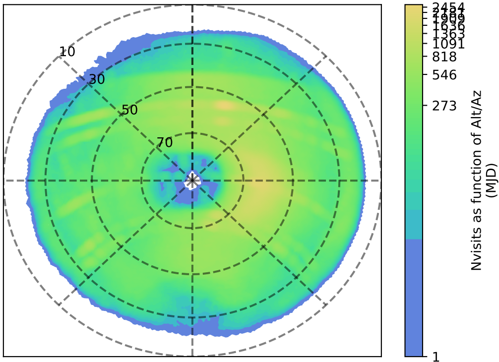
too_elab_r64_d3_griz_v3.4_10yrs z: Nvisits as function of Alt/Az
