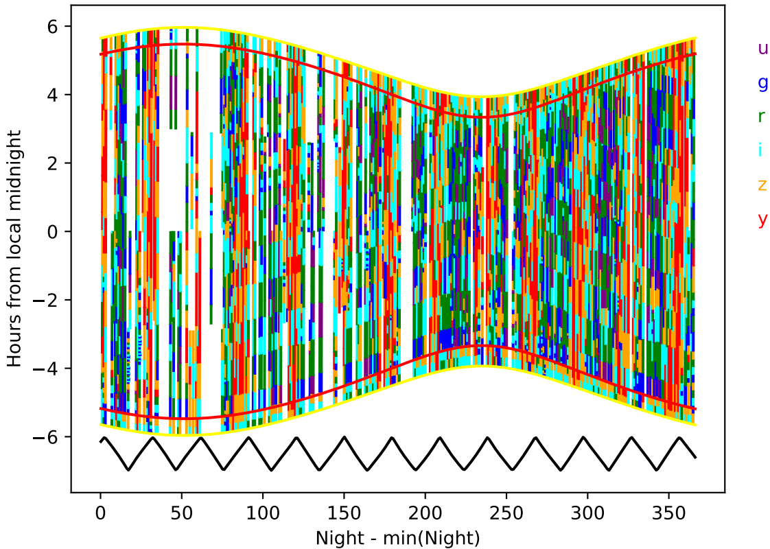
too_elab_r64_d3_griz_v3.4_10yrs year 9-10: Hourglass
