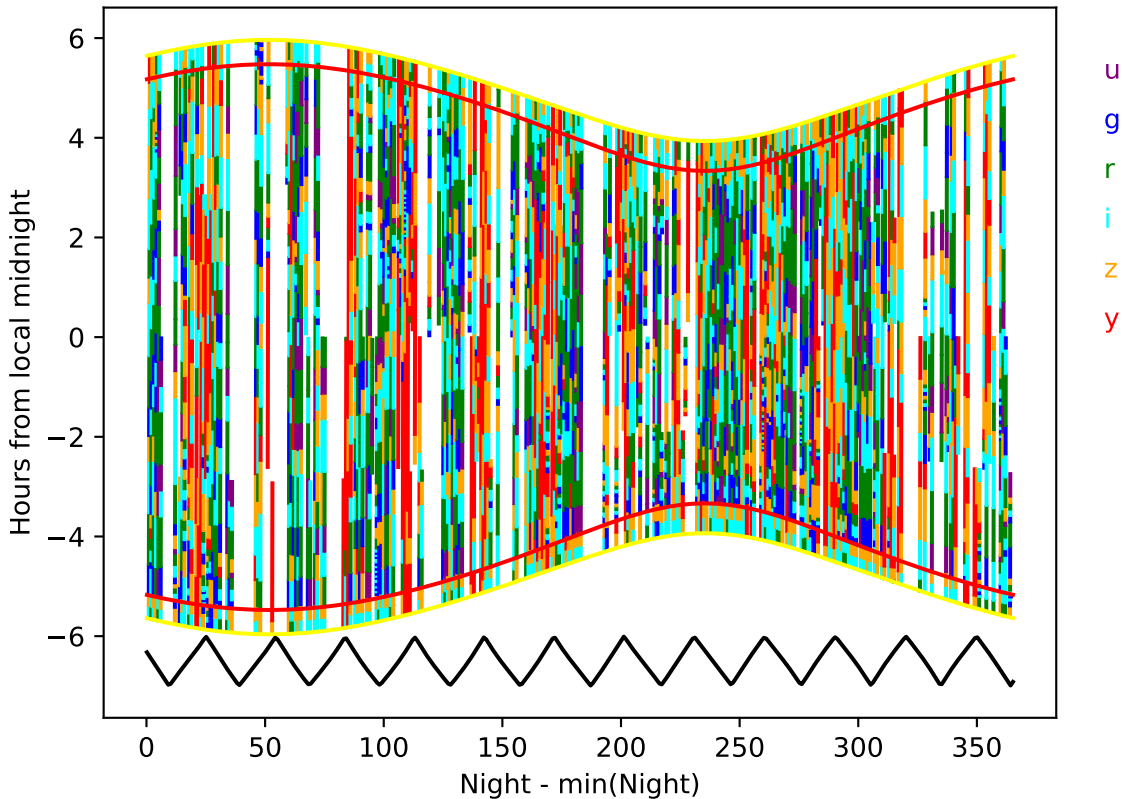
too_elab_r64_d3_griz_v3.4_10yrs year 7-8: Hourglass
