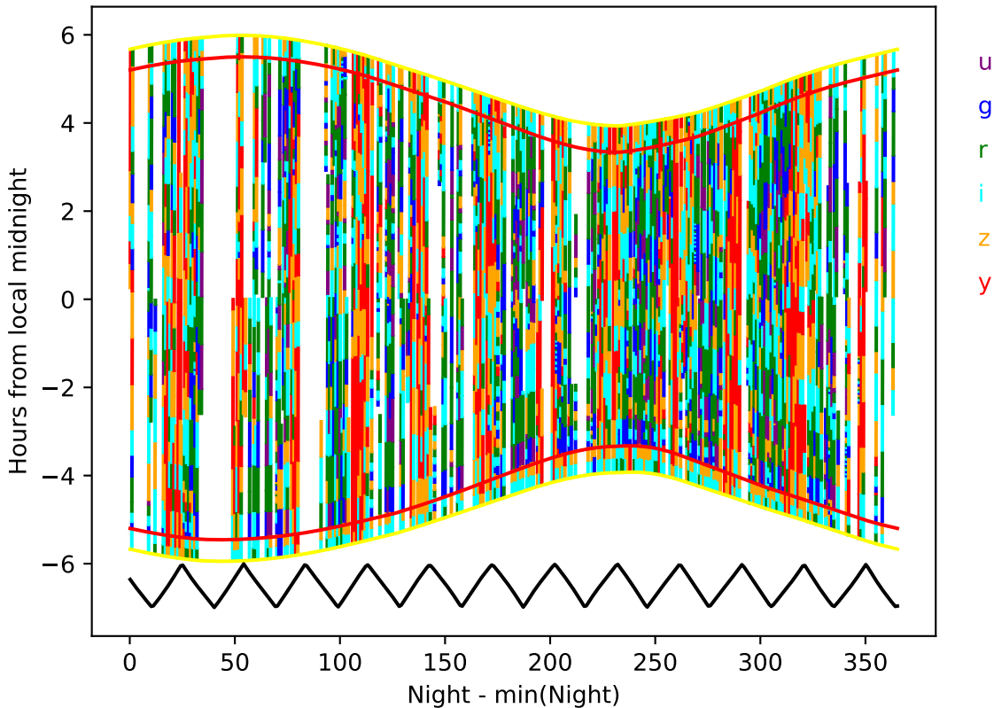
too_elab_r64_d3_griz_v3.4_10yrs year 4-5: Hourglass
