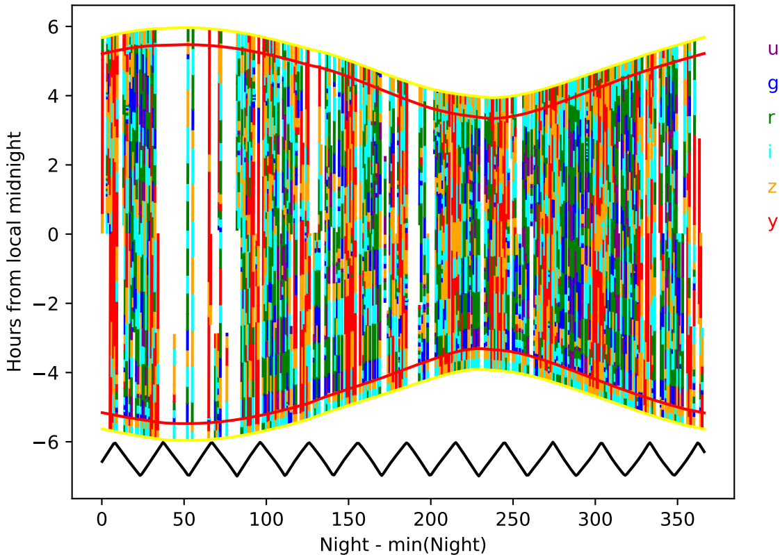
too_elab_r64_d3_griz_v3.4_10yrs year 3-4: Hourglass
