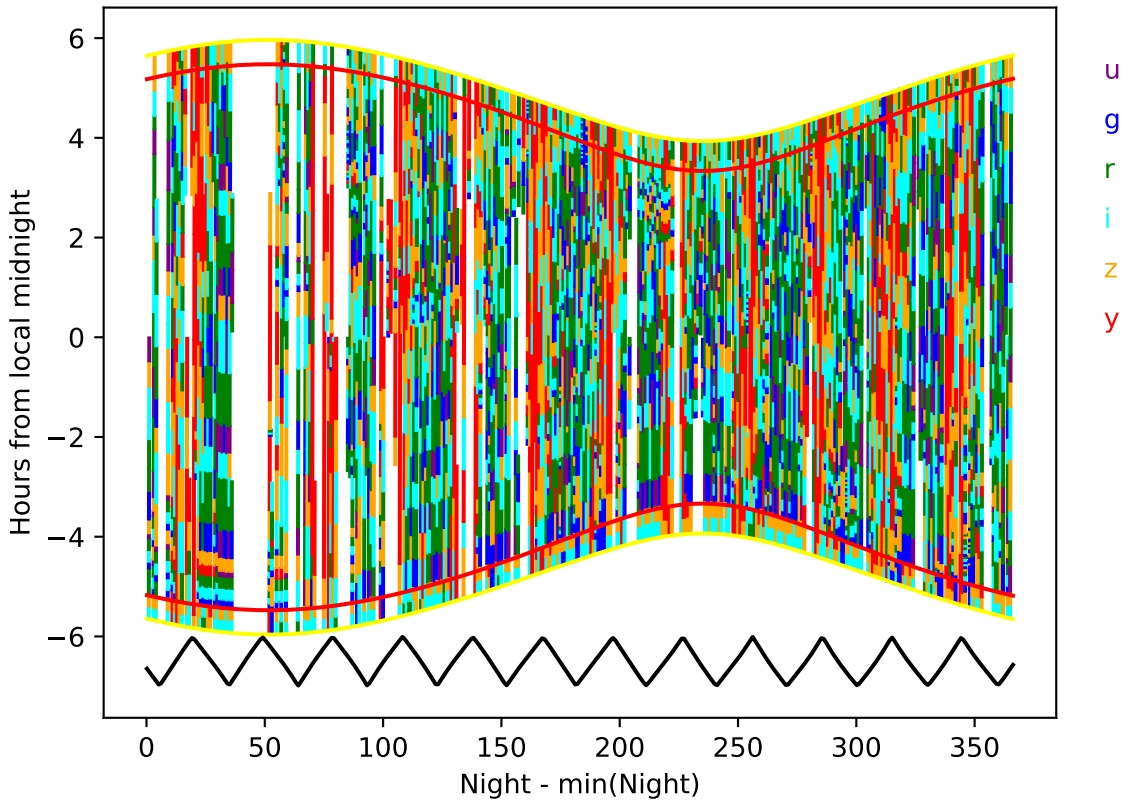
too_elab_r64_d3_griz_v3.4_10yrs year 2-3: Hourglass
