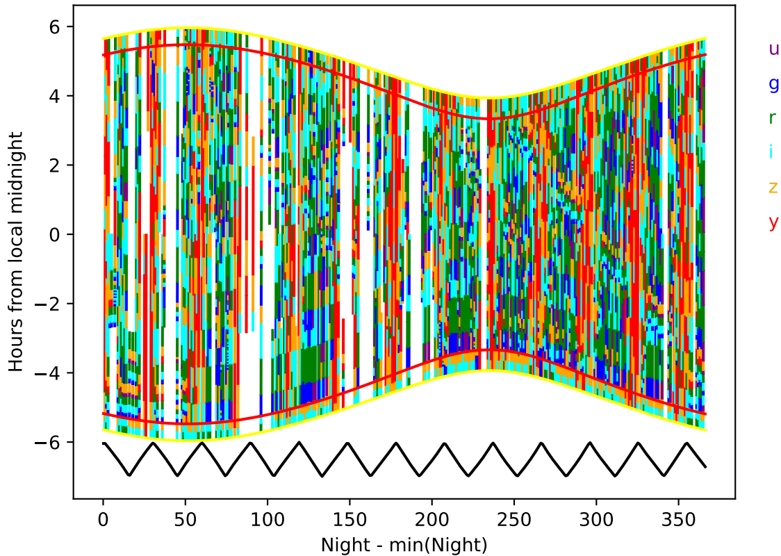
too_elab_r64_d3_griz_v3.4_10yrs year 1-2: Hourglass
