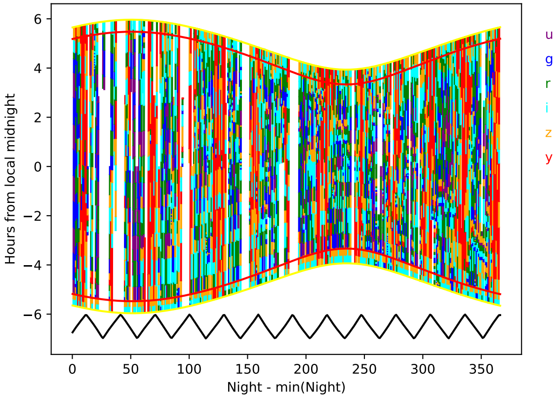
too_elab_r64_d3_griz_v3.4_10yrs year 0-1: Hourglass
