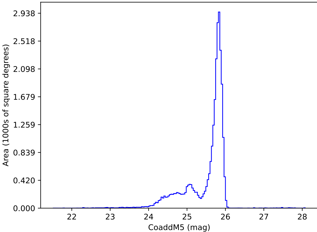
too_elab_r64_d3_griz_v3.4_10yrs z: CoaddM5
