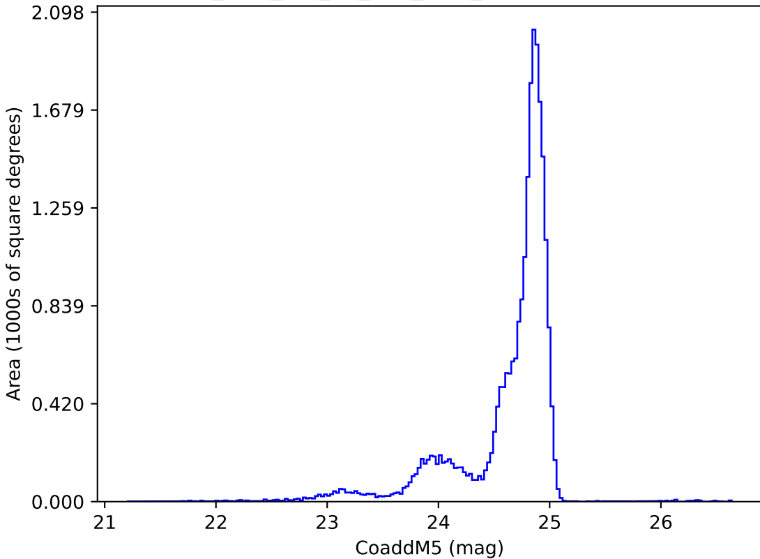
too_elab_r64_d3_griz_v3.4_10yrs y: CoaddM5
