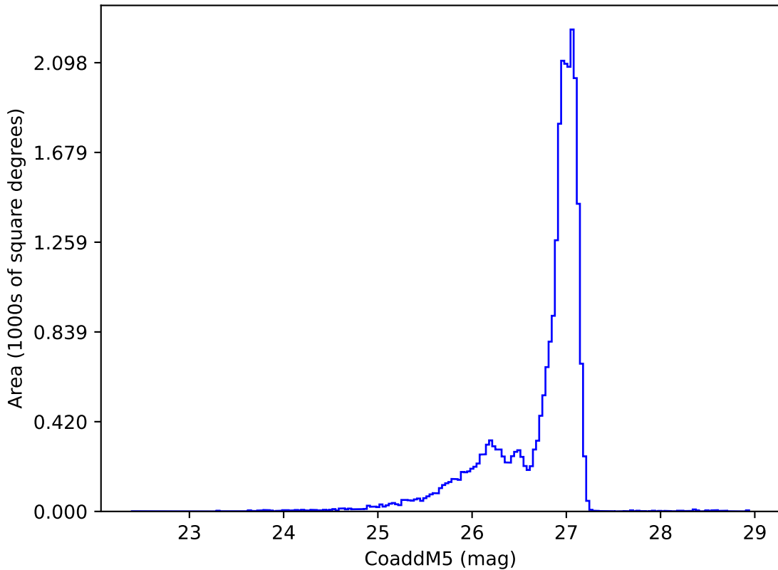
too_elab_r64_d3_griz_v3.4_10yrs r: CoaddM5
