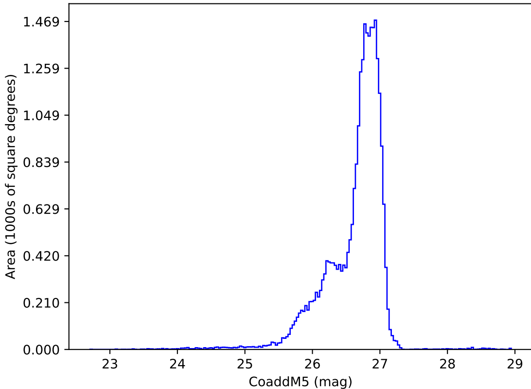
too_elab_r64_d3_griz_v3.4_10yrs g: CoaddM5
