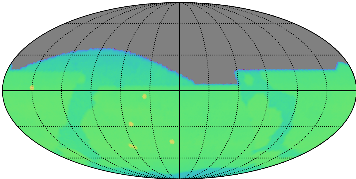
too_elab_r64_d3_griz_v3.4_10yrs : CoaddM5
