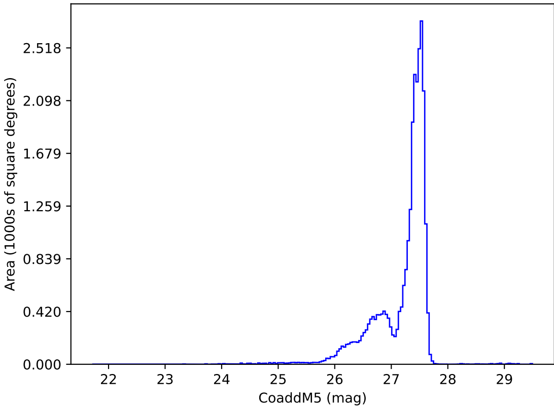
too_elab_r64_d3_griz_v3.4_10yrs : CoaddM5
