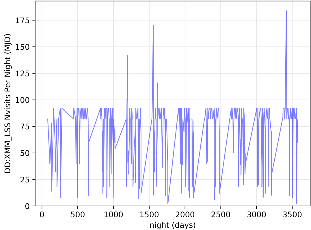
too_elab_r64_d3_griz_v3.4_10yrs all bands: DD:XMM_LSS Nvisits Per Night
