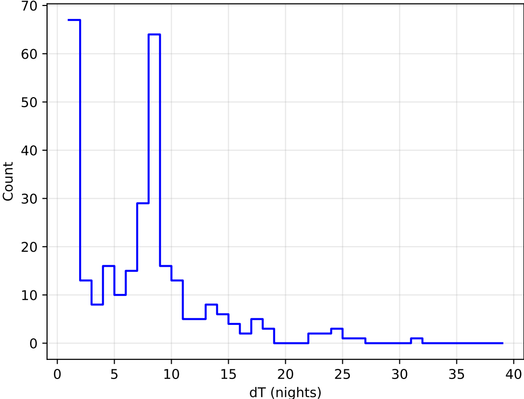
too_elab_r64_d3_griz_v3.4_10yrs all bands: DD:XMM_LSS Delta Nights Histogram
