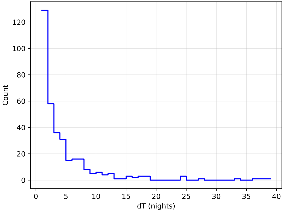
too_elab_r64_d3_griz_v3.4_10yrs all bands: DD:WFD Delta Nights Histogram
